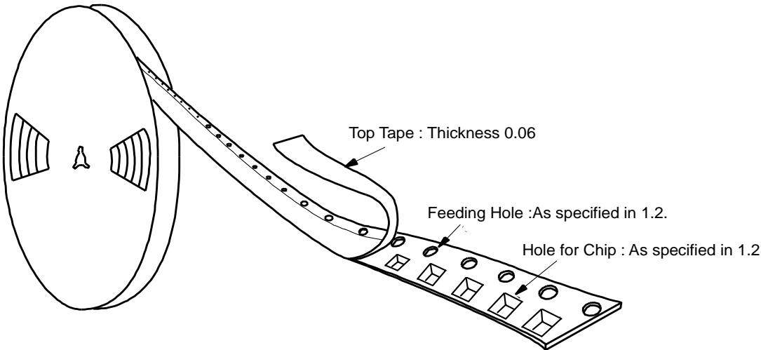
Fig.3 Taping Diagram
