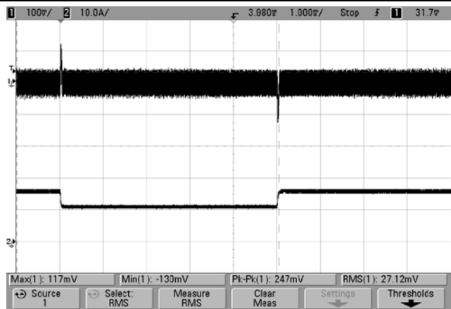
Step Load Transient Response@25°C
