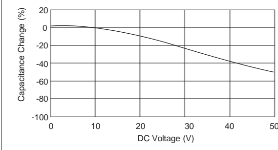
[Example of DC Voltage Characteristics]
