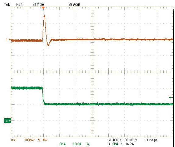
Step Load Transient Response (Vin=7V, Vout=0.69V, Cload=188µF, Iout=20A to 10A) Trace 1=Vout, 100 mV/div(AC), Trace 4=Iout, 10A/div.
