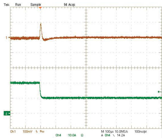
Step Load Transient Response (Vin=12V, Vout=3.3V, Cload=188µF, Iout=20A to 10A) Trace 1=Vout, 100 mV/div(AC), Trace 4=Iout, 10A/div.
