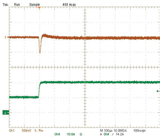
Step Load Transient Response (Vin=12V, Vout=3.3V, Cload=188µF, Iout=10A to 20A) Trace 1=Vout, 100 mV/div(AC), Trace 4=Iout, 10A/div.
