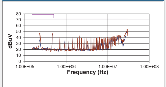
NCS1S2403SC
