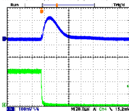
Step Load Transient Response (Vin=12V, Vout=5V, Cload=12x10µF X5R 0805 ceramic, total 120µF, Iout=1.5A to 0A) Top trace=Vout, Bottom trace=Iout
