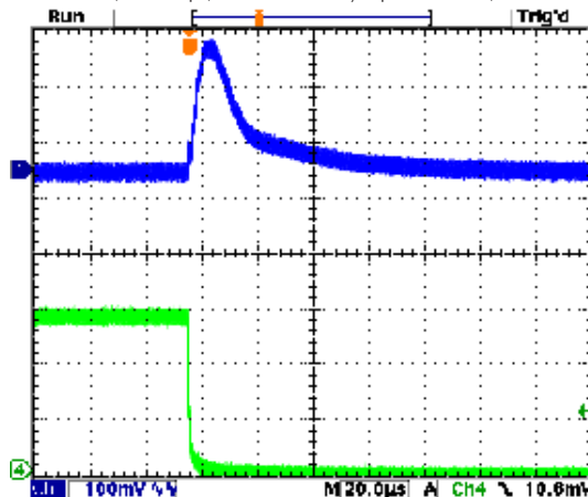
Step Load Transient Response (Vin=7.5V, Vout=5V, Cload=5x10µF X5R 0805 ceramic, total 50µF, Iout=1.5A to 0A) Top trace=Vout, Bottom trace=Iout
