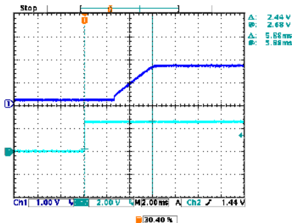
On/Off Enable Startup (Vin=12V, Vout=1.5V, Iout=1.5A, Cload=0) Channel 2=Enable, Channel 1=Vout
