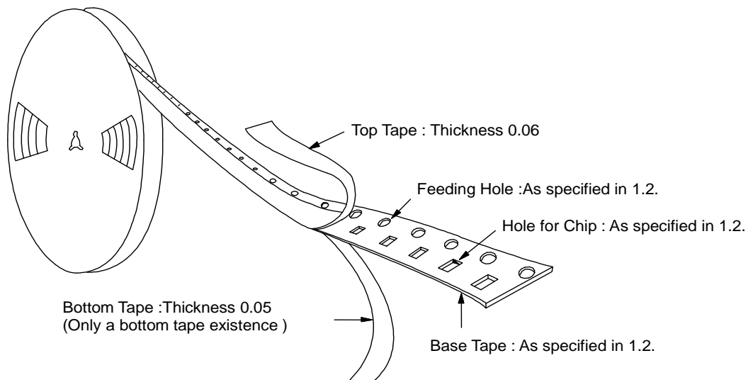
Fig.3 Taping Diagram
