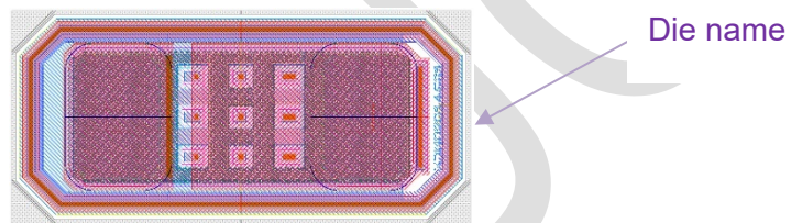
Figure 6 – Layout view
