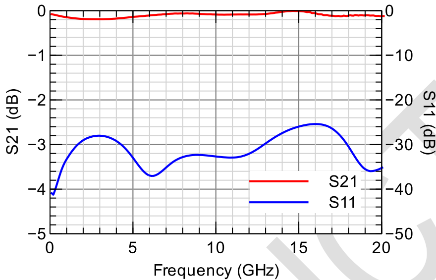
Figure 2 – 5.6nF ULSC measurement results (module of S-parameters)
