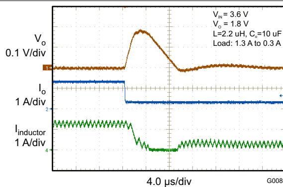
图 18. Typical Application (PFM Mode)
