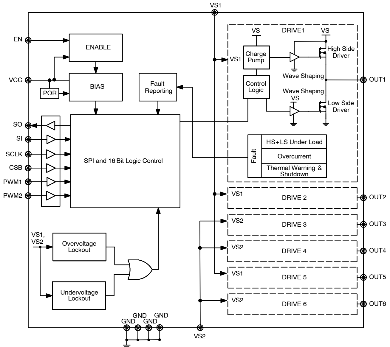
Figure 2. Block Diagram
