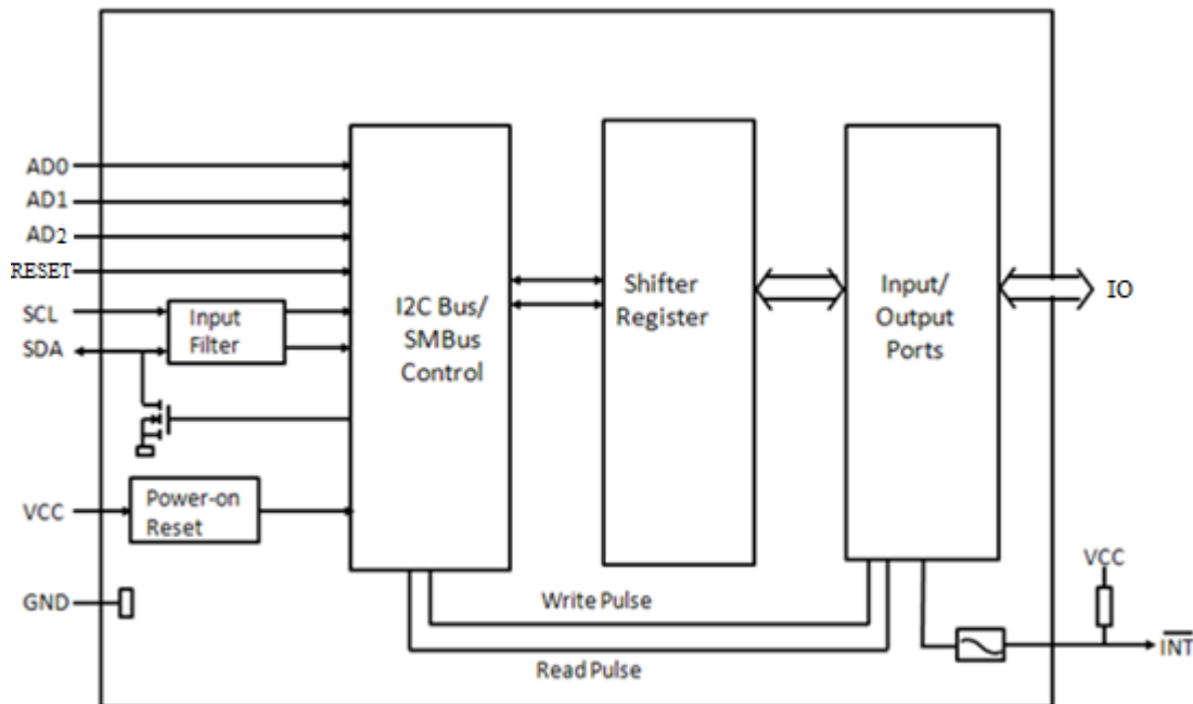
Fig 2: Block diagram
