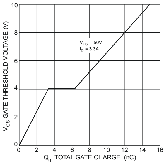
Figure 10 Gate Charge
