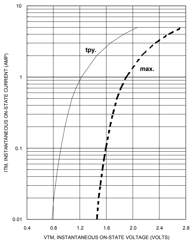
Figure 4. On-State Characteristics
