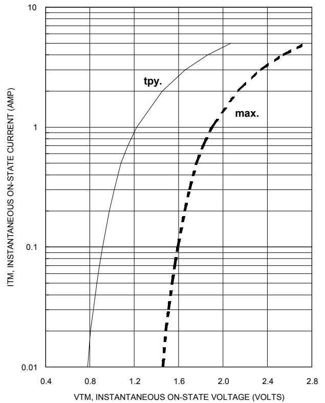
Figure 4. On-State Characteristics
