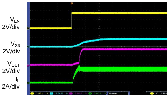
Time 10ms/div
