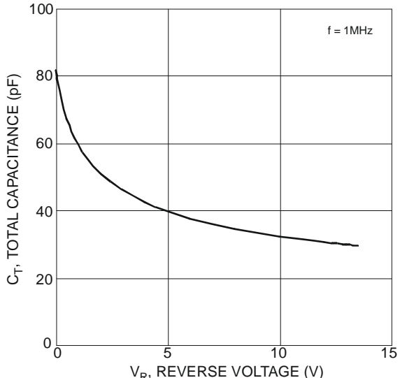
Figure 4 Typical Capacitance
