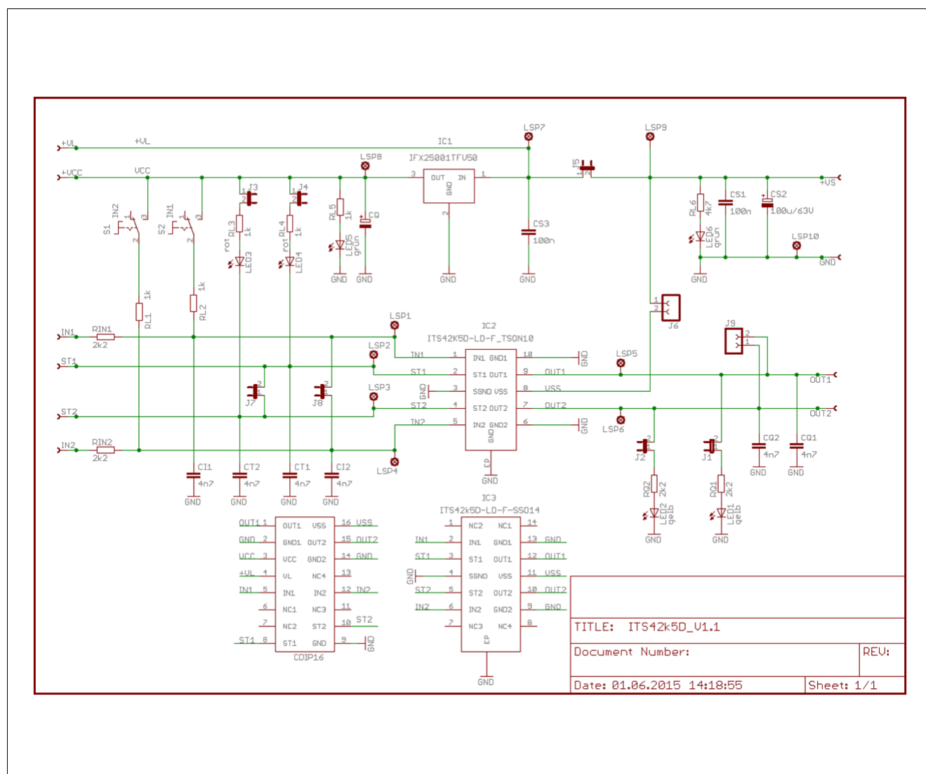
Figure 4 Schematic of ITS42k5D-LD-F Demo board (PG-TSO-10)
