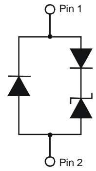
Device Schematic
