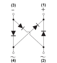
Internal Schematic
