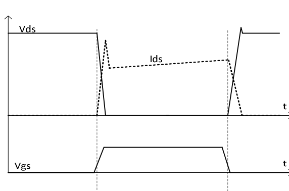
Figure 26 Typical Reverse Channel Recovery
