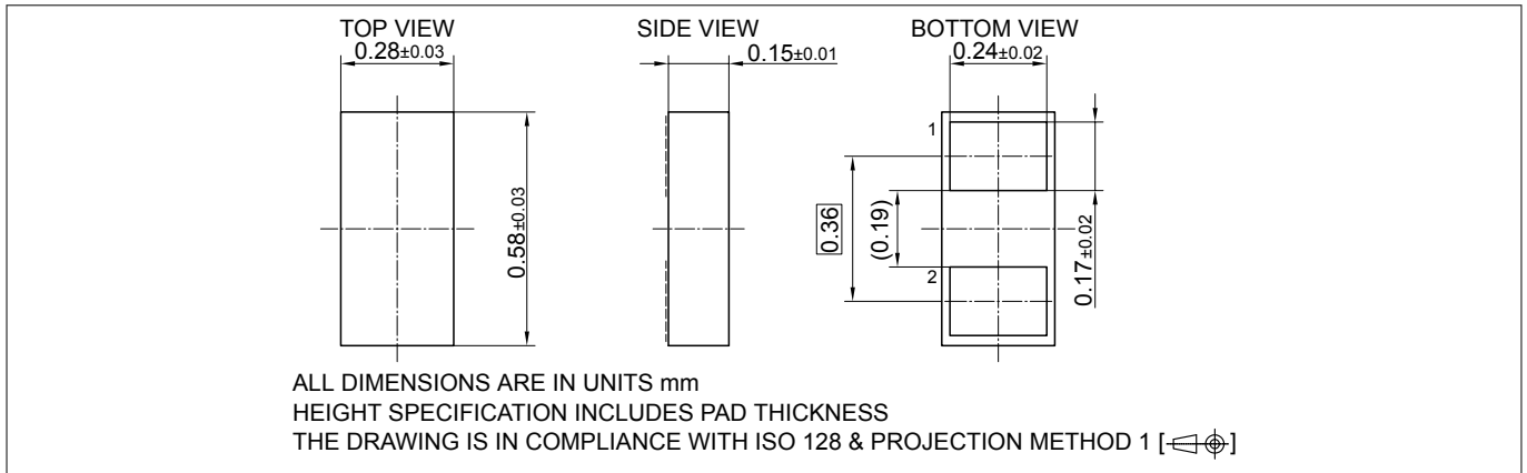
Figure 10 WLL-2-3 package
