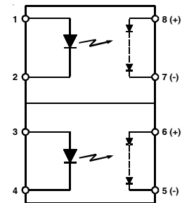
Connection Diagram
