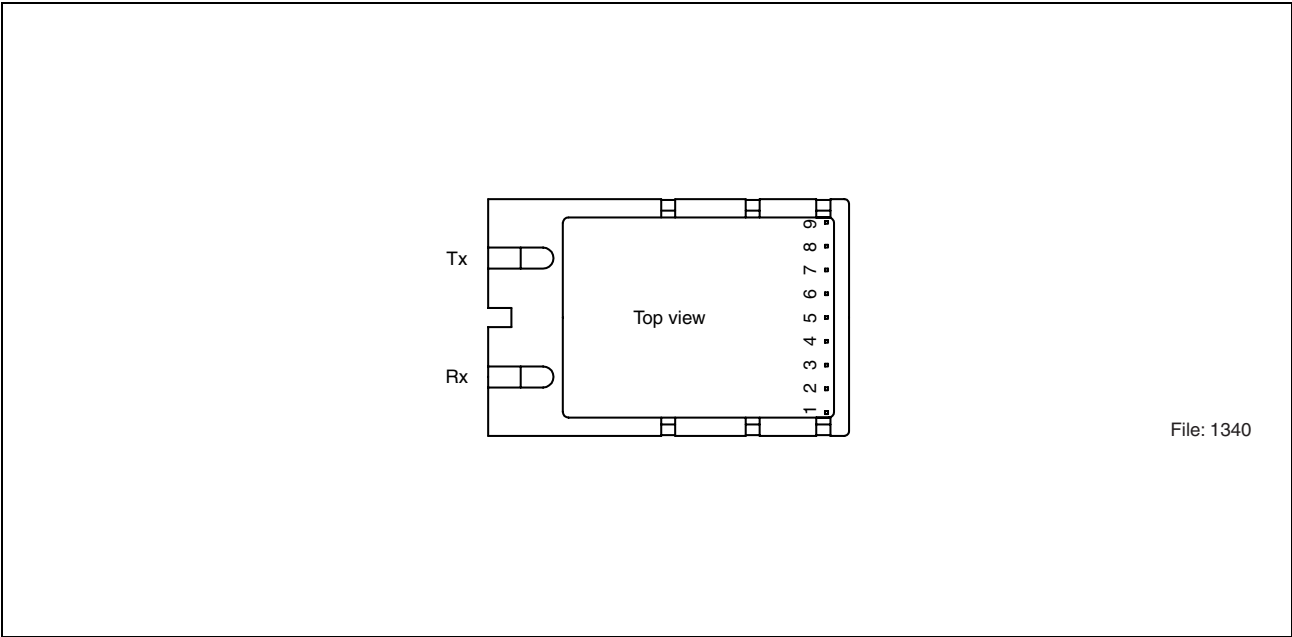
Figure 1 V23826-C18-C
