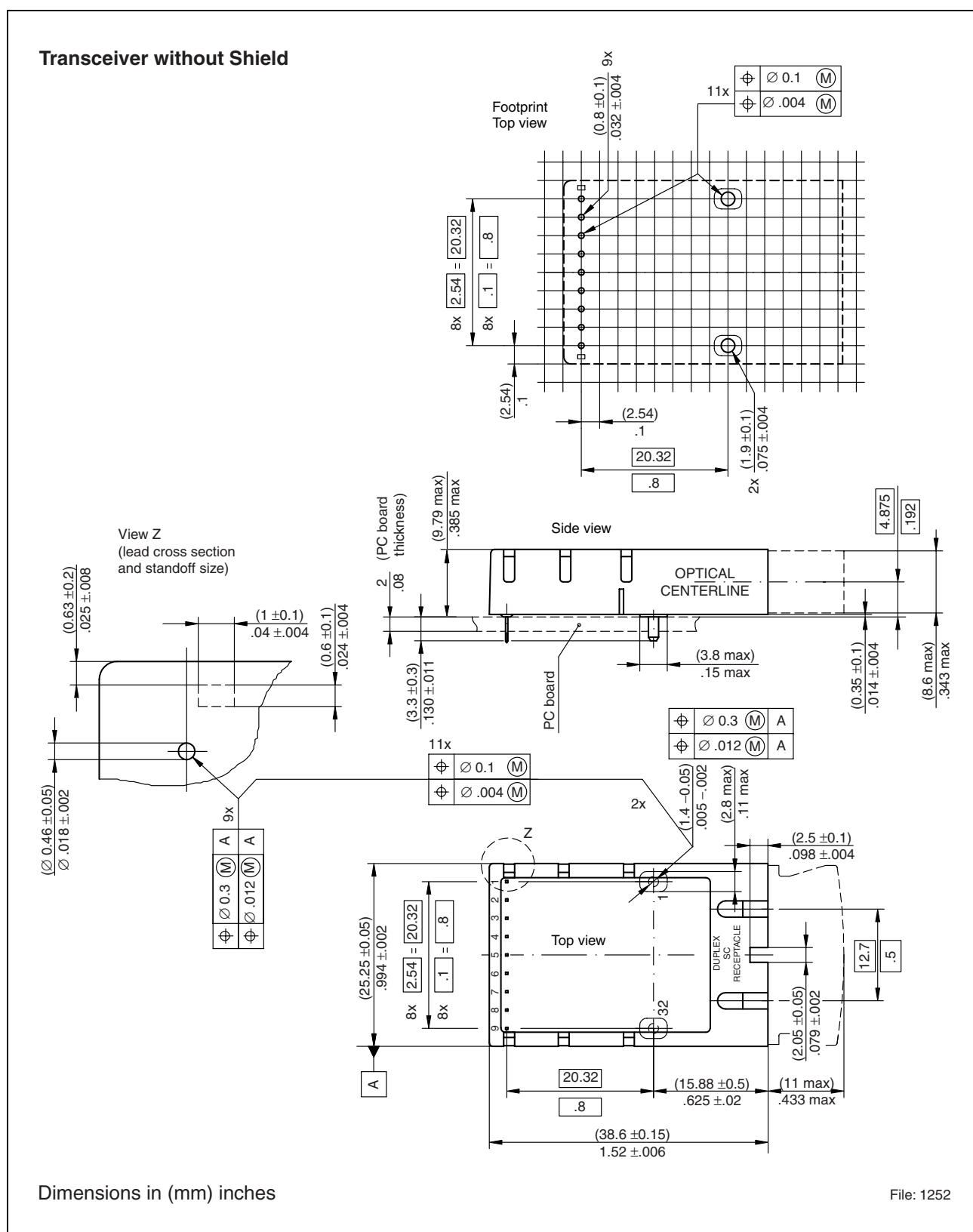
Figure 9 V23826-C18-C
