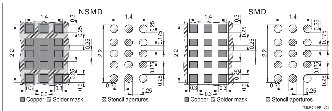
Figure 4 Footprint TSLP-7-4
