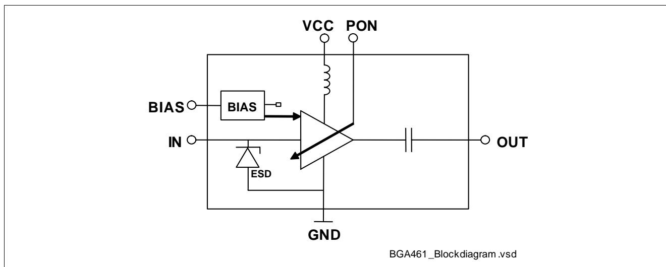
Figure 1 Blockdiagram
