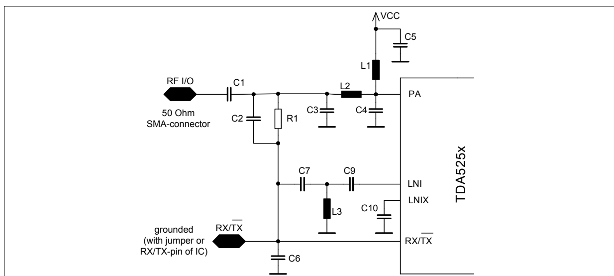
Figure 3-2 RX-Mode
