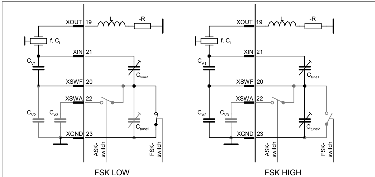
Figure 3-14 FSK modulation
