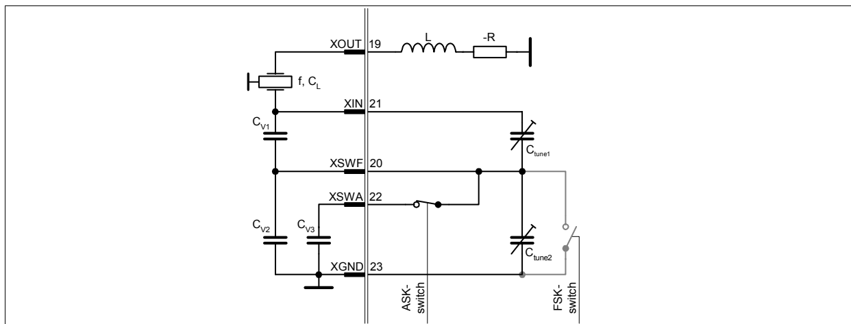
Figure 3-15 FSK receive
