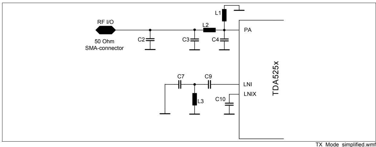
Figure 3-5 TX_Mode_simplified
