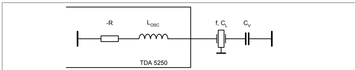
Figure 3-12 Crystal Oscillator
