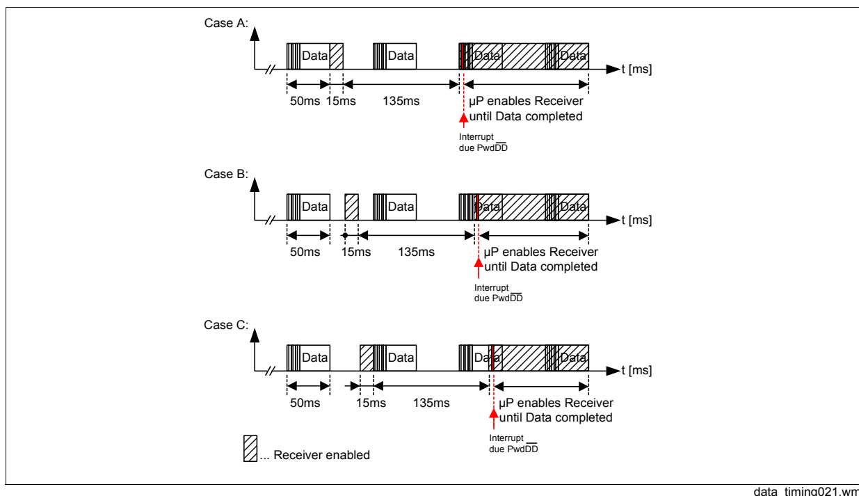
Figure 3-32 3 possible timings
