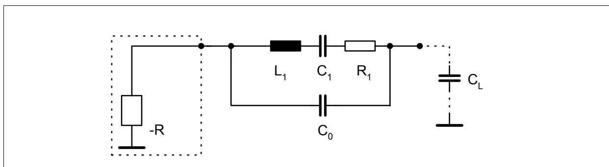
Figure 3-11 Crystal
