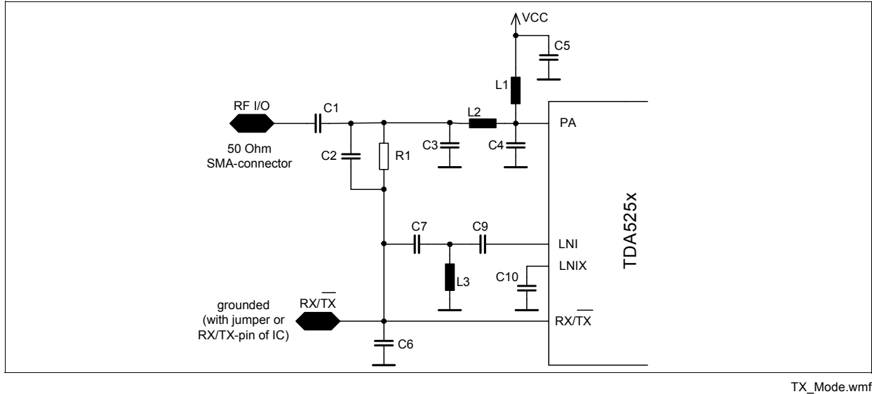
Figure 3-4 TX_Mode
