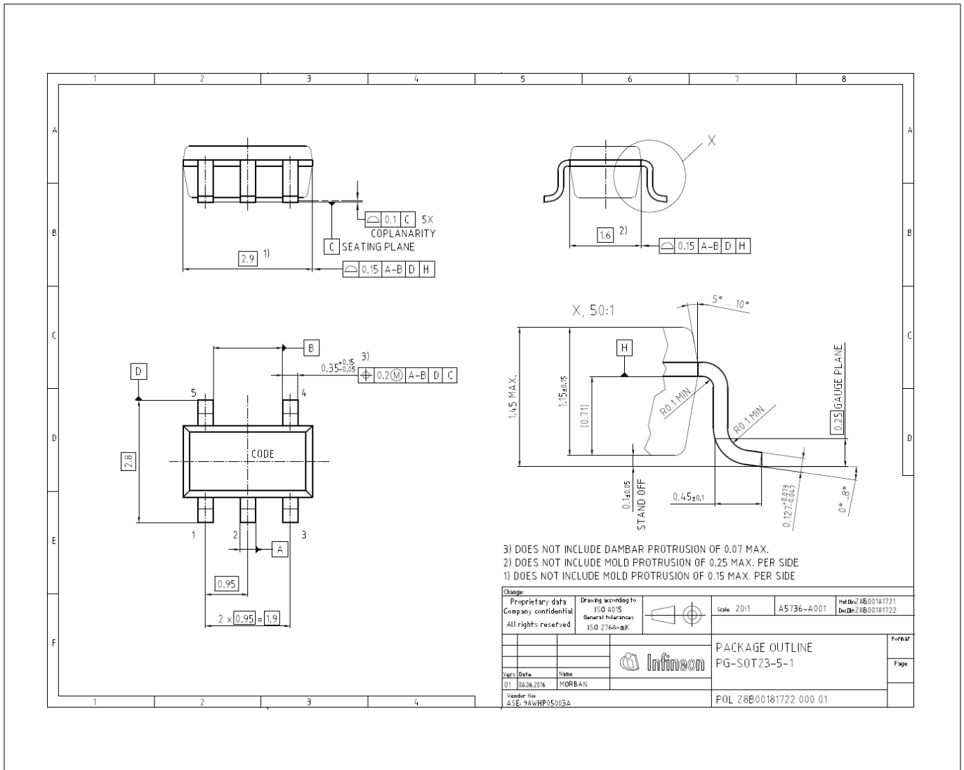
Figure 15 Package Outline PG-SOT23-5-1
