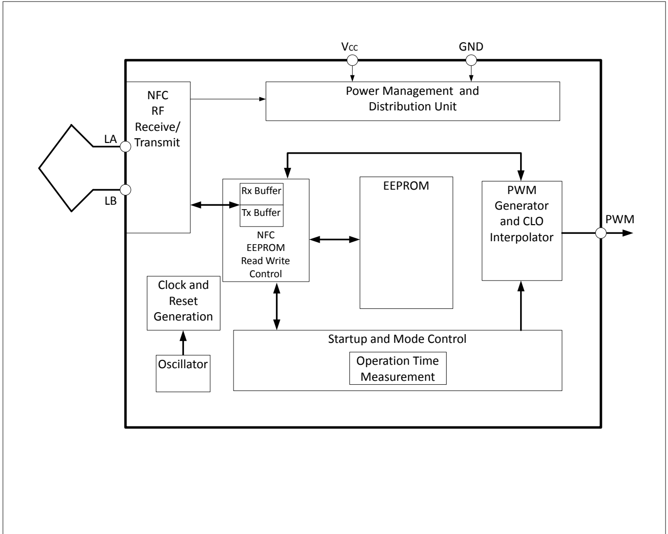
Figure 3 Block Diagram
