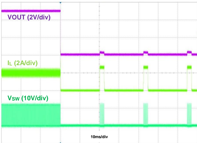
Figure 12. Output Short Protection, I_{OUT} = 2\text{A}
