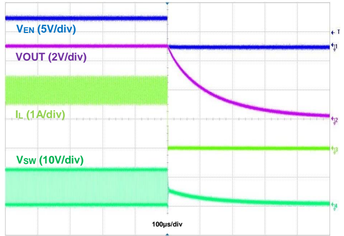
Figure 11. Shutdown Using EN, I_{OUT} = 2\text{A}
