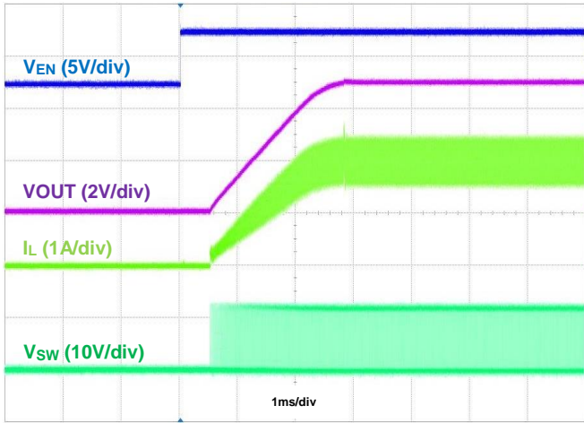
Figure 10. Startup Using EN, I_{OUT} = 2\text{A}
