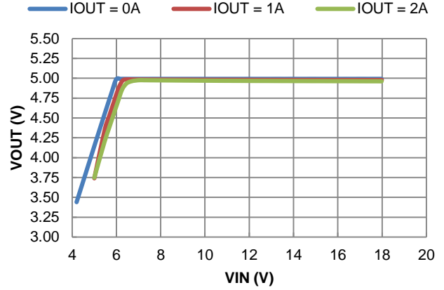
Figure 27. Line Regulation
