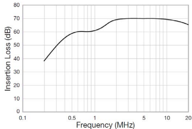
LF-305
