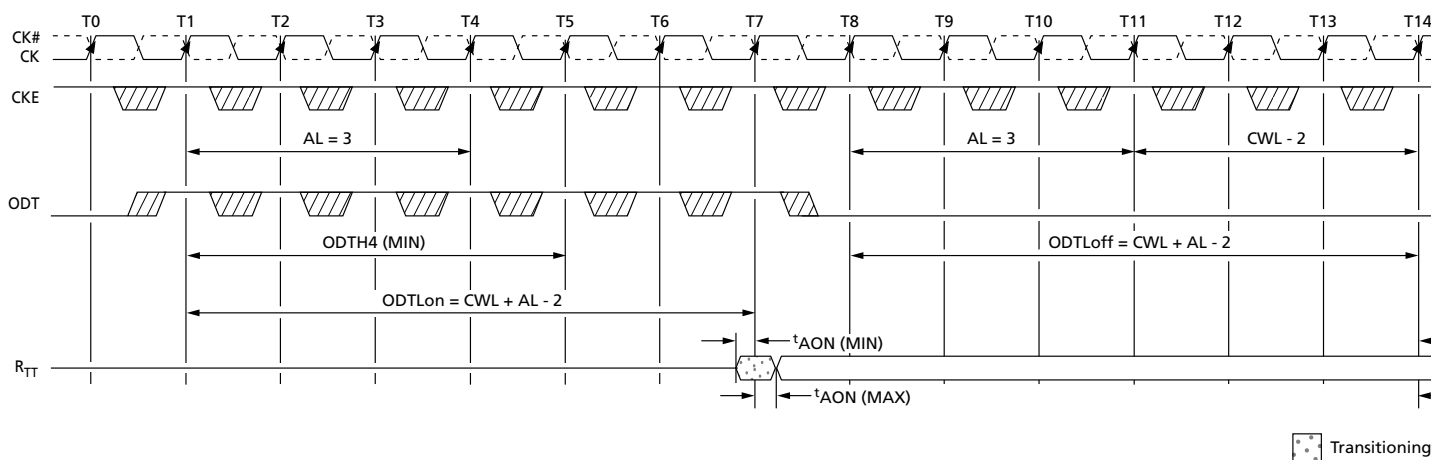
Figure 111: Synchronous ODT
