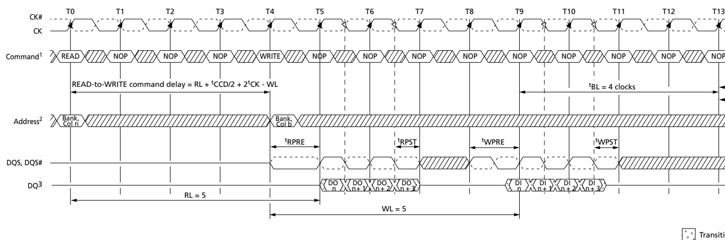
Figure 69: READ (BC4) to WRITE (BC4) OTF
