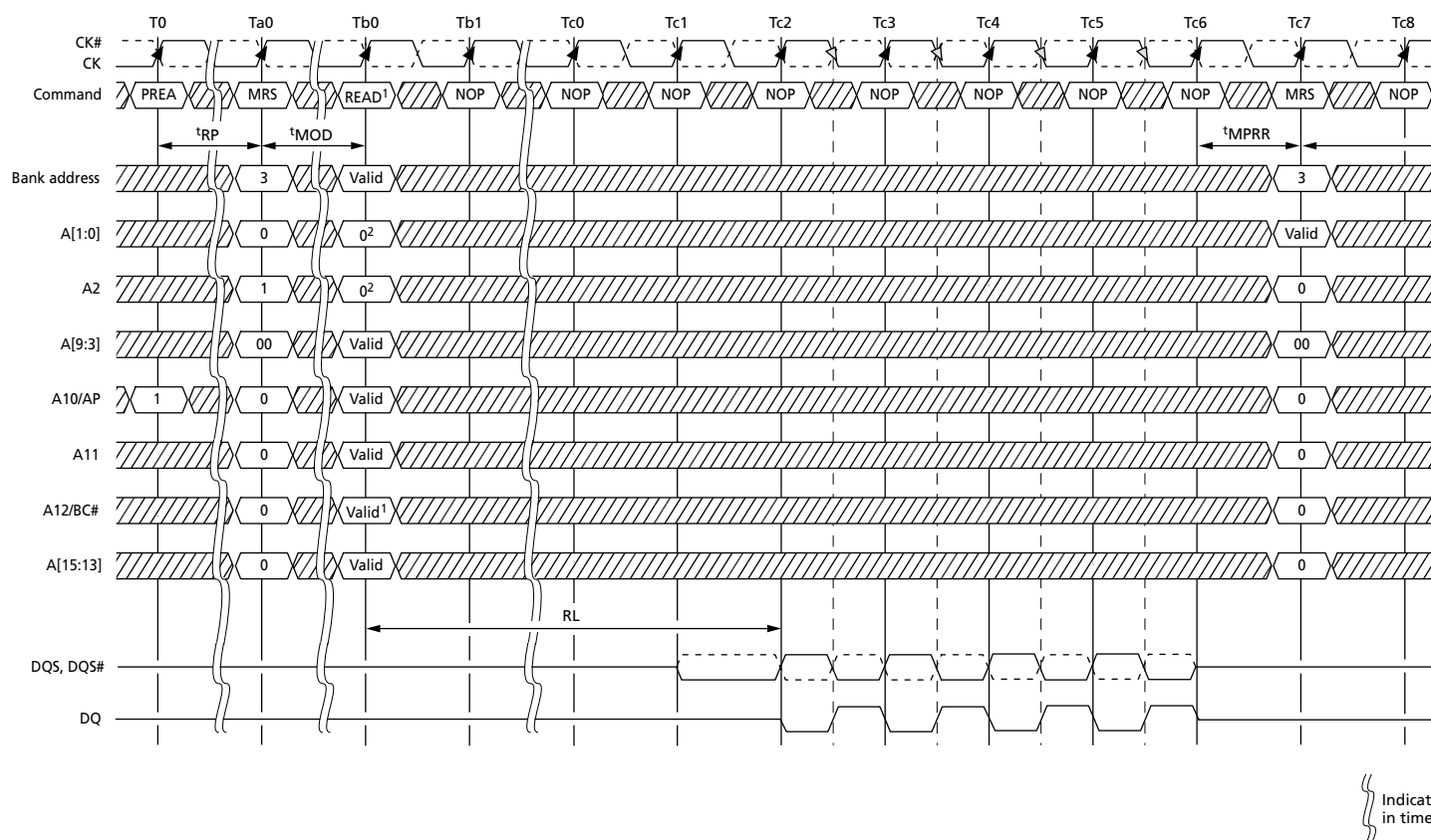
Figure 57: MPR System Read Calibration with BL8: Fixed Burst Order Single Readout
