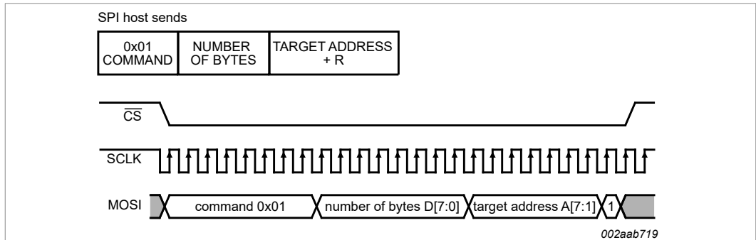
Figure 9. Read N bytes from I 2 C-bus target device
