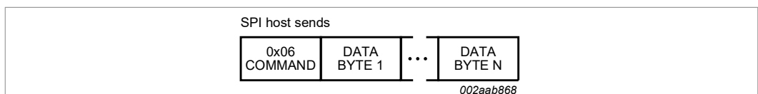
Figure 11. Read buffer
