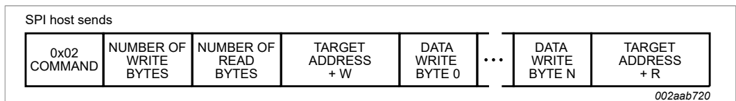
Figure 10. I 2 C-bus read after write
