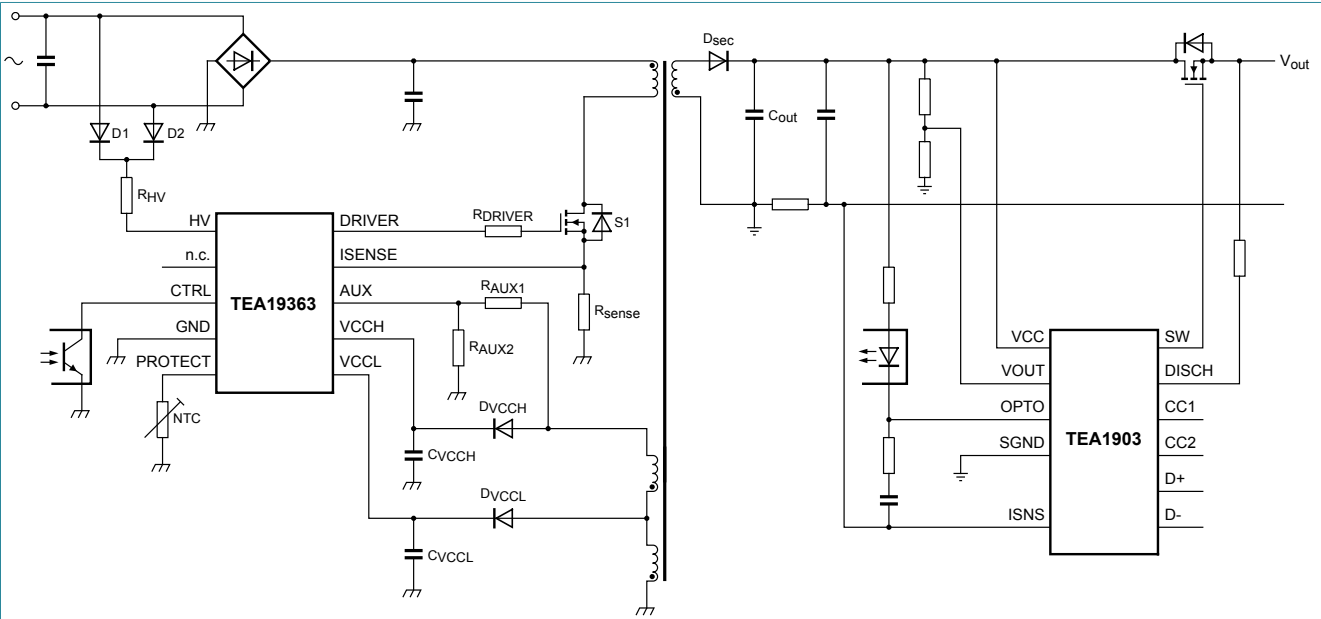
Figure 23. TEA19363LT application diagram with TEA1903T
