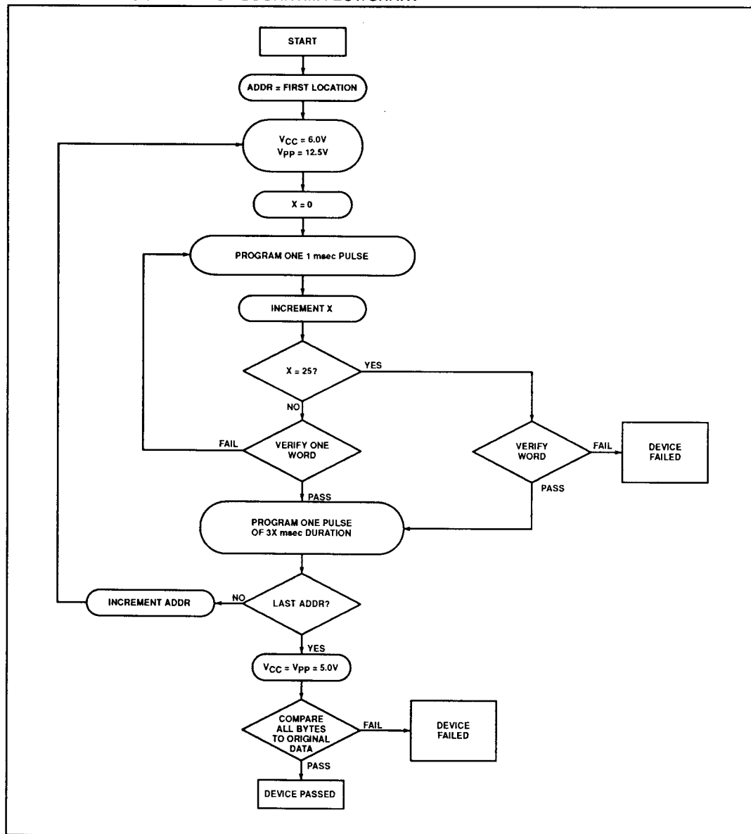
INTELLIGENT PROGRAMMING ALGORITHM FLOWCHART
