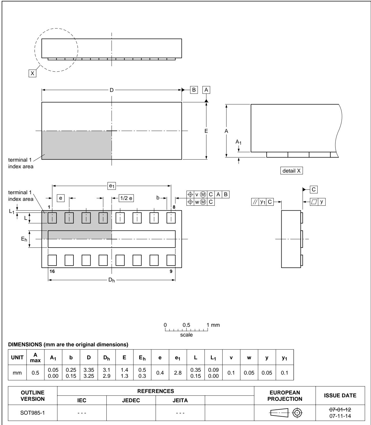
Fig 6. Package outline SOT985-1 (HXSON16U)
