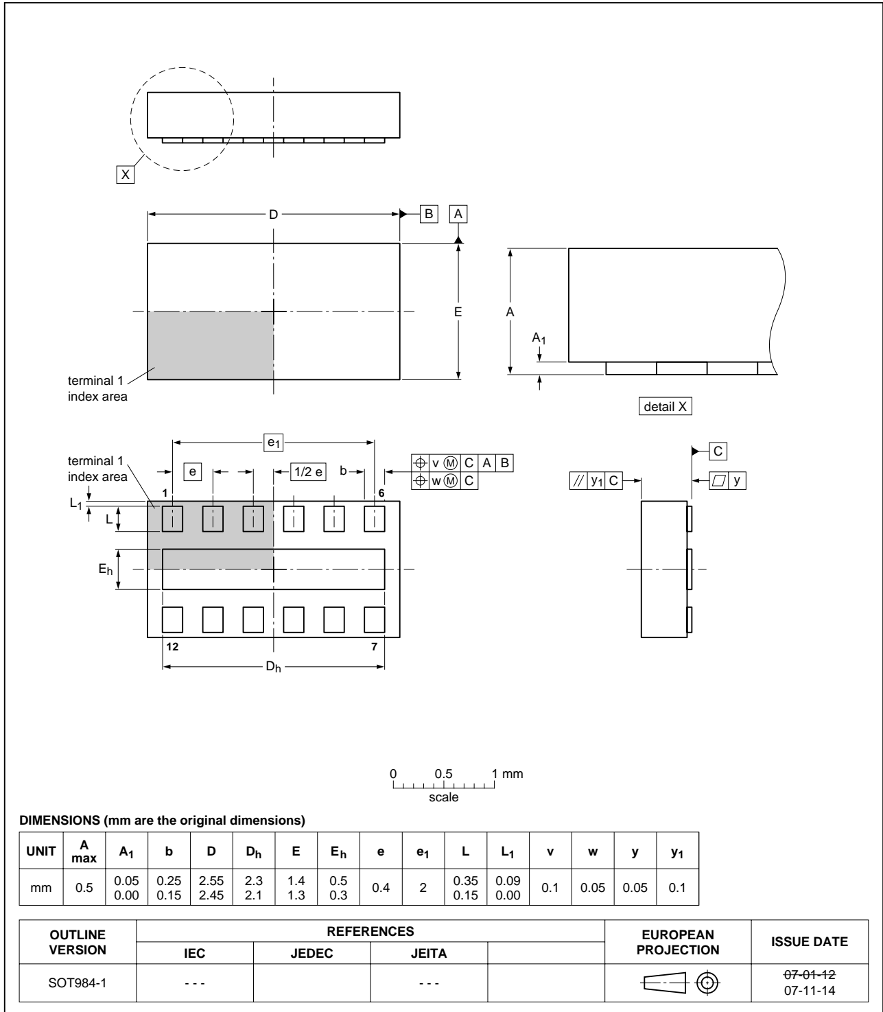
Fig 5. Package outline SOT984-1 (HXSON12U)
