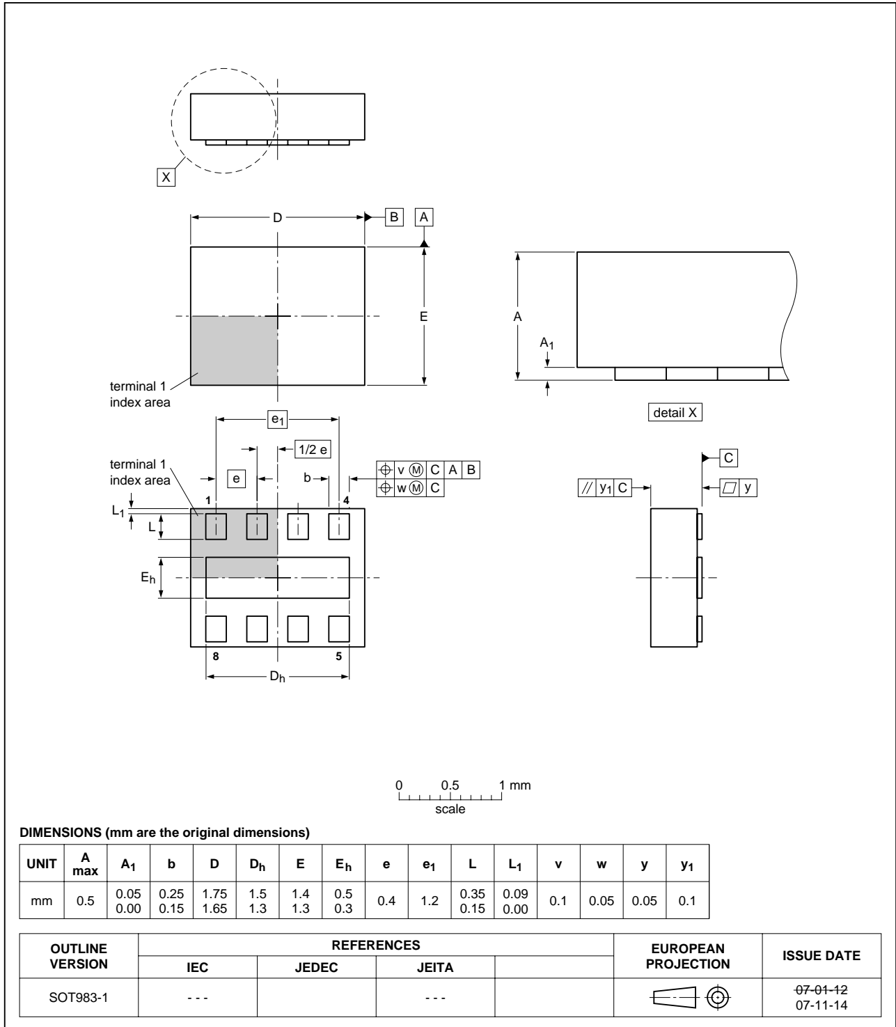
Fig 4. Package outline SOT983-1 (HXSON8U)
