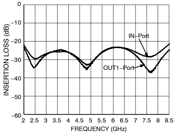
Figure 4. Return Loss vs Frequency IN-OUT1 ON, CTL1 = 0 V, CTL2 = 2.7 V
