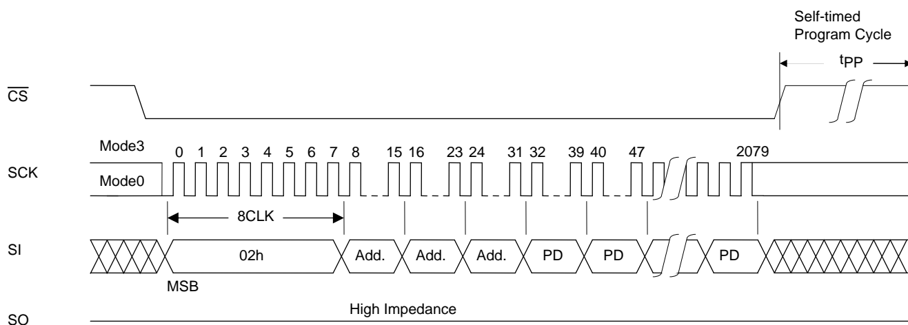
Figure 14 Page Program
