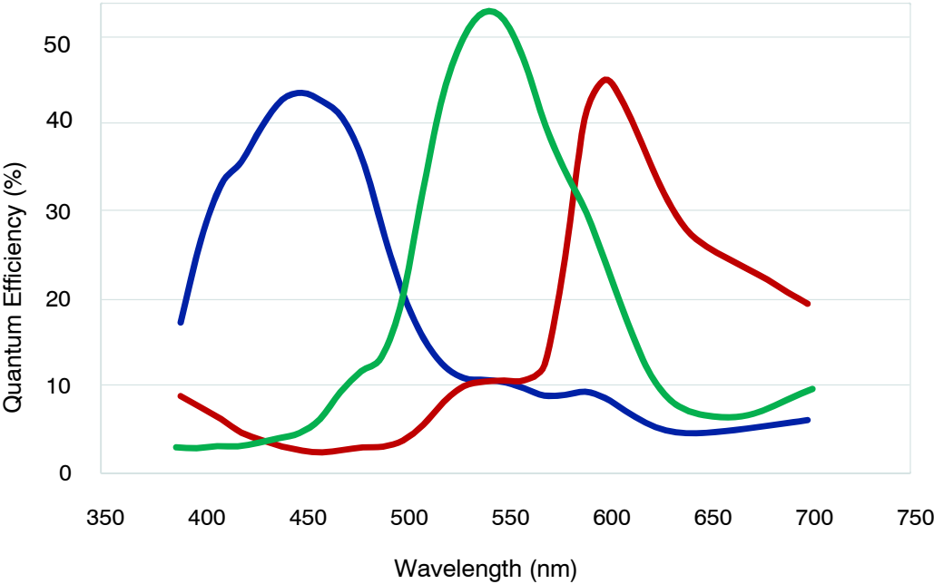
Figure 27. Quantum Efficiency
