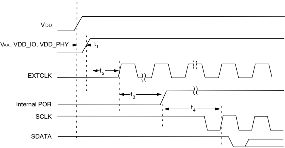
Figure 29. Power-Up Sequence
