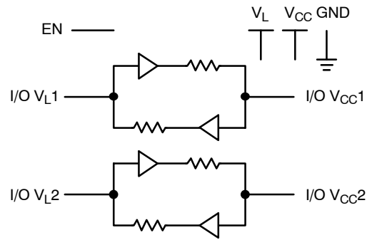
Figure 5. Logic Diagram
