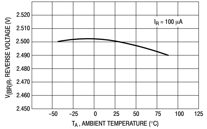
Figure 11. Temperature Drift
