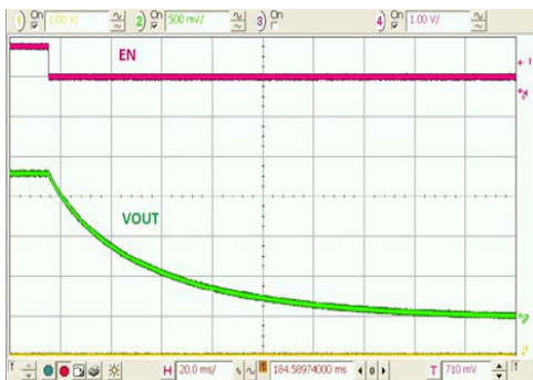
Figure 26. Shutdown, 10 k \Omega Load, No Output Discharge
