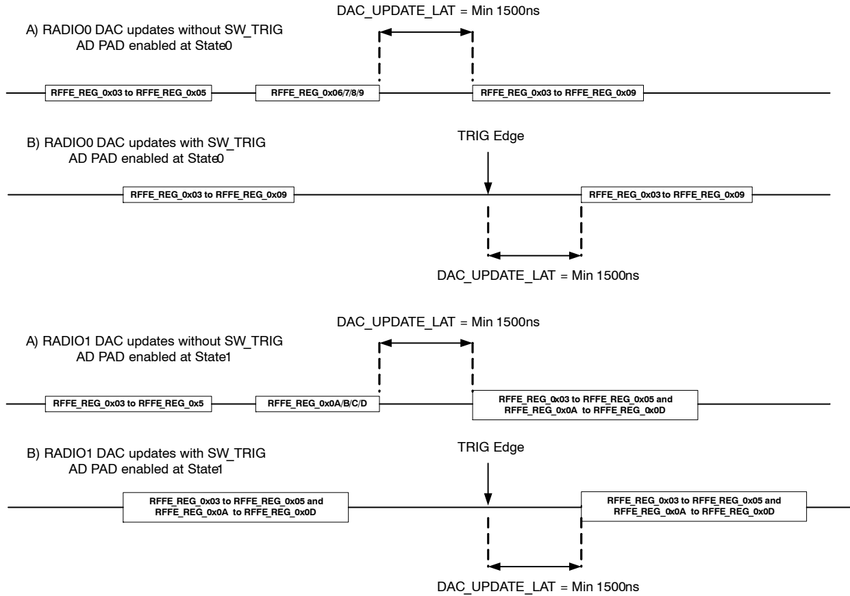
Figure 10. DAC_UPDATE_LAT Requirement
