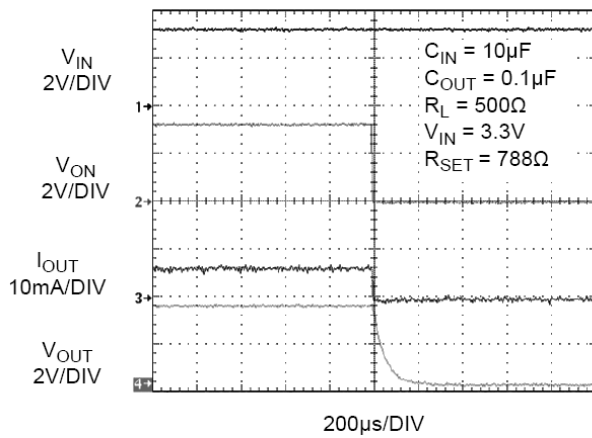
Figure 19. t_{OFF} Response
