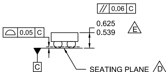
SIDE VIEWS
