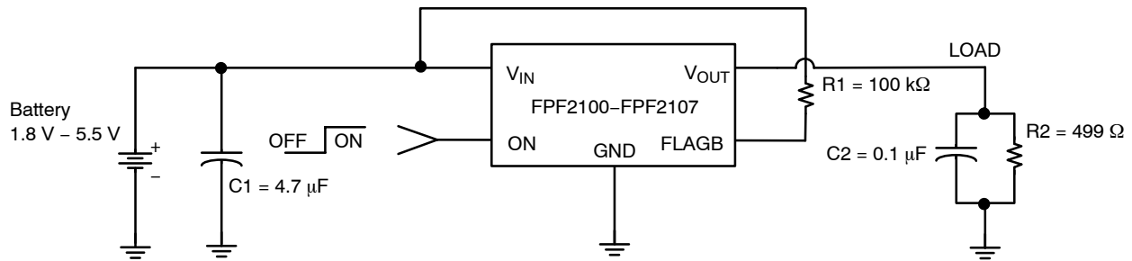
Figure 25. Typical Application
