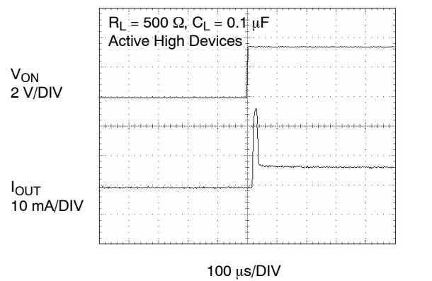
Figure 20. T_{\text{ON}} Response
