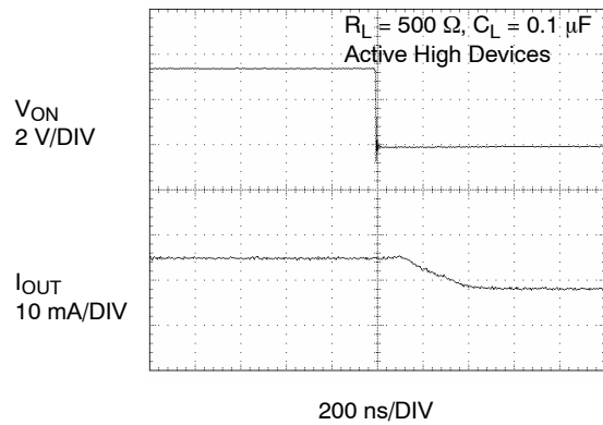
Figure 21. T_{\text{OFF}} Response
