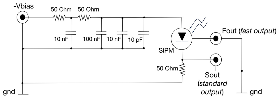
Figure 7. Schematic of SMA Biasing Board
