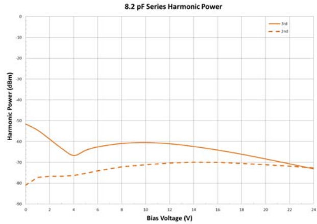
Figure 3. Harmonic Power*
