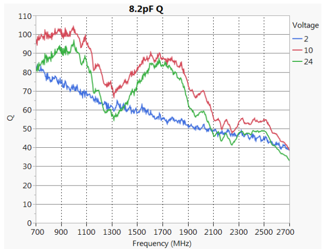
Figure 5. Q*
