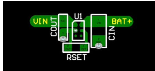
Figure 12. Example Layout, FAN54120UC (CSP)
