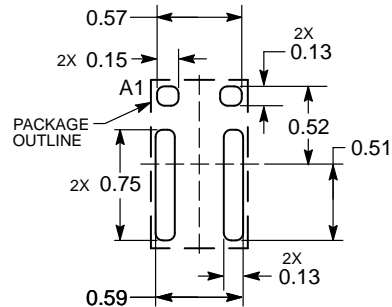
DIMENSIONS: MILLIMETERS
