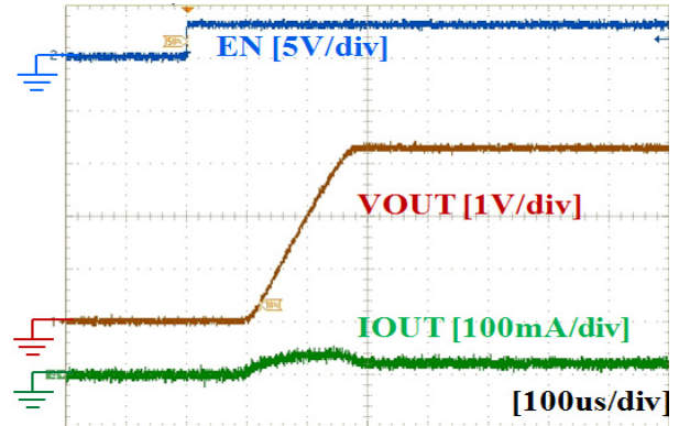
Figure 26. Turn-On Response (VIN = 3.3 V, CIN = 1 µF, COUT = 1 µF, RL = 150 Ω, SEL = LOW)
