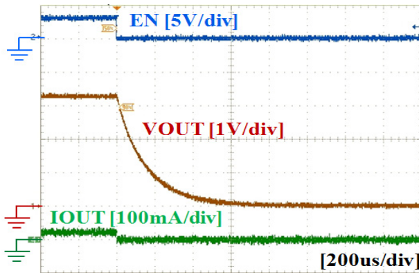
Figure 27. Turn-Off Response with FPF1320 (VIN = 3.3 V, CIN = 1 µF, COUT = 1 µF, RL = 150 Ω, SEL = LOW)
