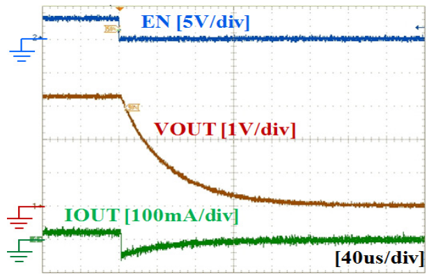
Figure 28. Turn-Off Response with FPF1321 (VIN = 3.3 V, CIN = 1 µF, COUT = 1 µF, RL = 150 Ω, SEL = LOW)
