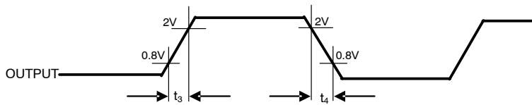
Figure 5. All Outputs Rise/Fall Time
