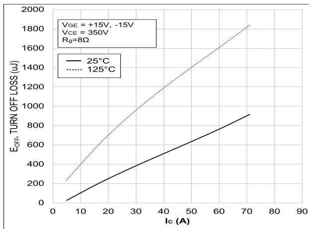
Figure 19. Typical Switching Loss E_{OFF} vs. I_C
