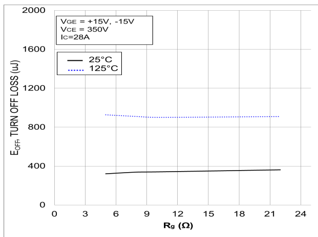
Figure 21. Typical Switching Loss E_{OFF} vs. R_g
